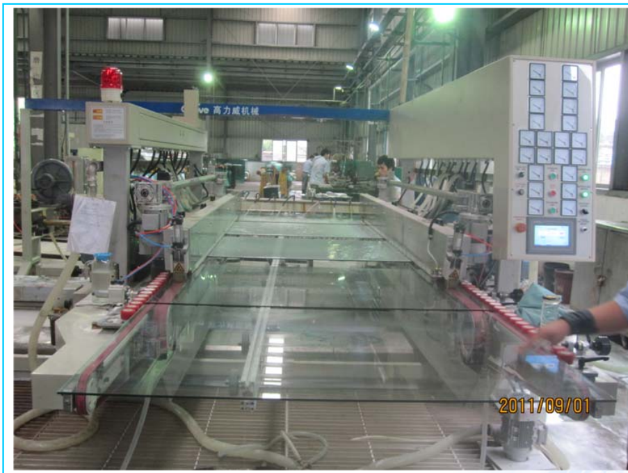
▲ New double edge polishing machine
